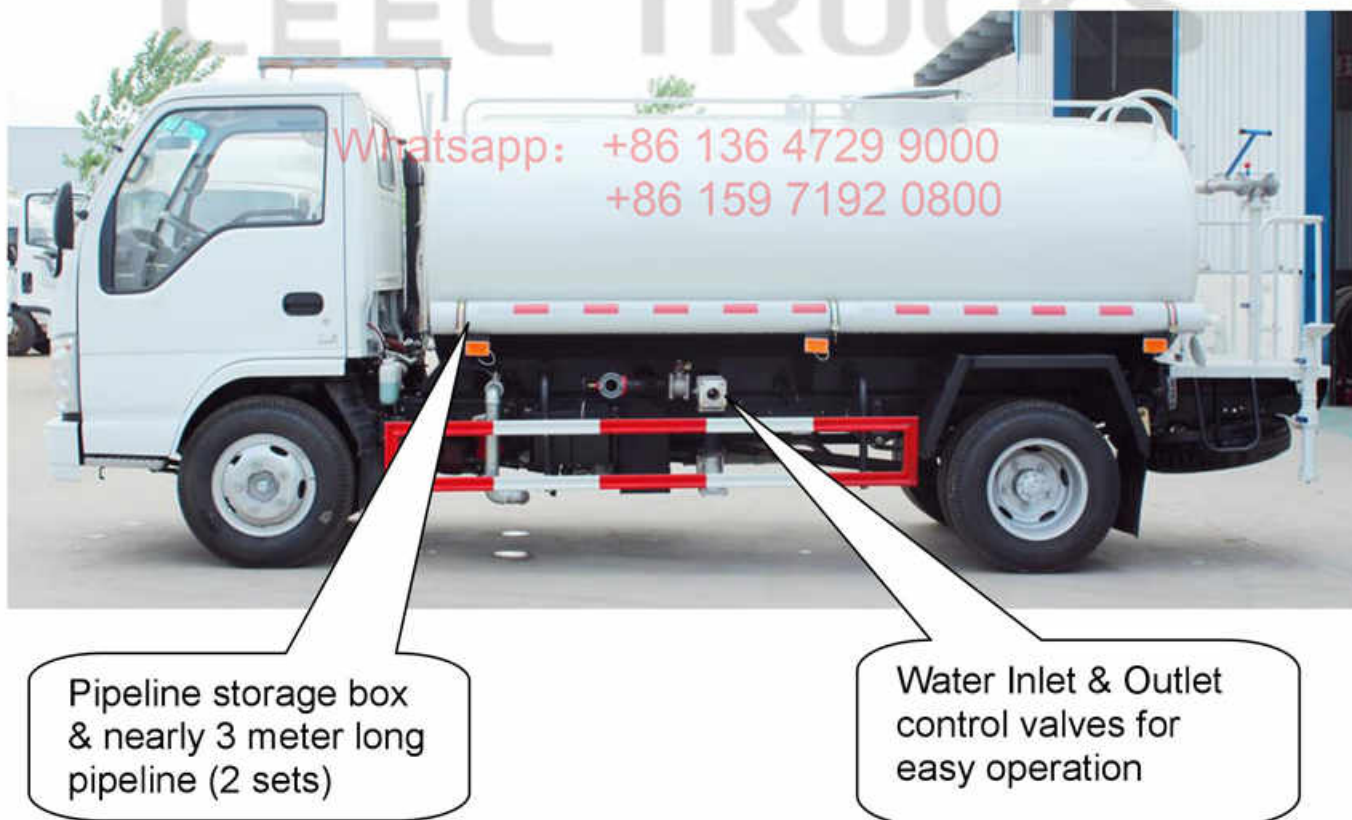
Side of the Tank: Pipeline storage box and Water pump system
